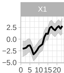
PreyNCC, 01.ZooPreyNCC, 01.Zoo
